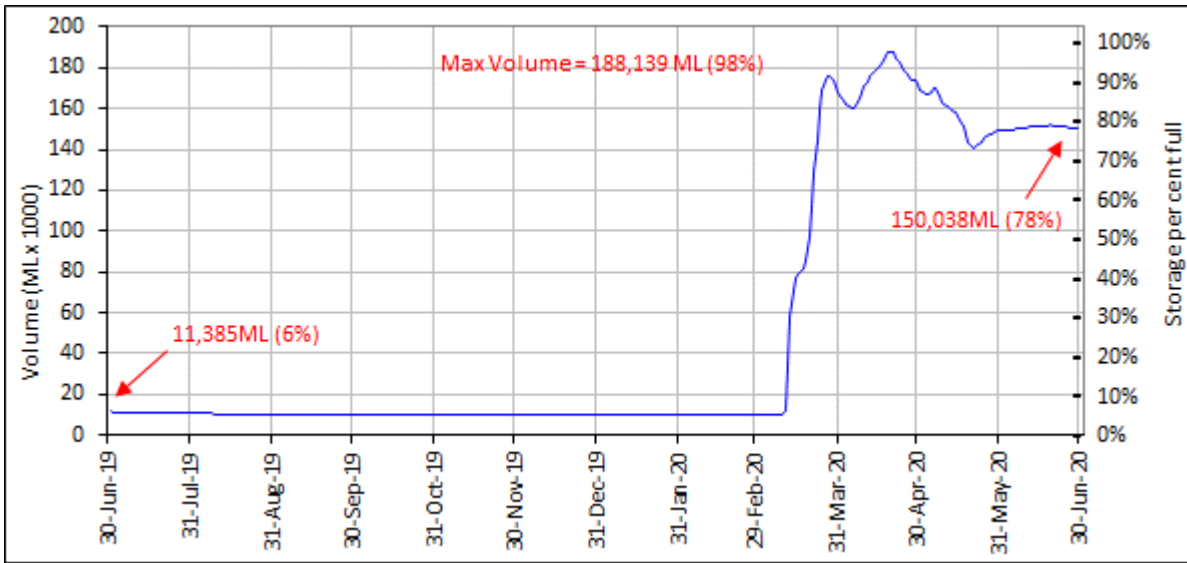
Figure 32: Lake Pamamaroo storage level and effective full storage capacity 2019–20
